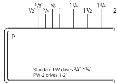
1" Wide Crown. 16 Gauge Staples. 1/2" - 1 1/4" Lengths. Capacity 140+.
